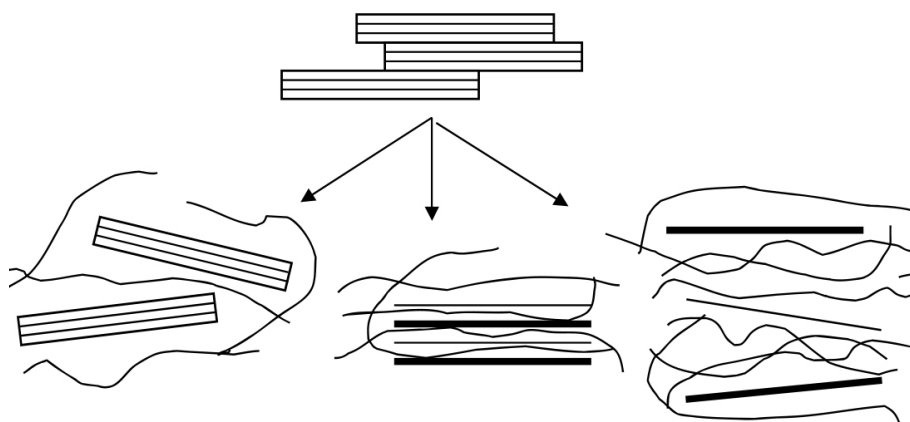
Figure 1. A common pictorial presentation of three types of polymer composites with clay (top). Bottom left, conventional composite; bottom center, intercalated nanocomposite; bottom right, exfoliated nanocomposite. After Refs [3, 8, 9].
