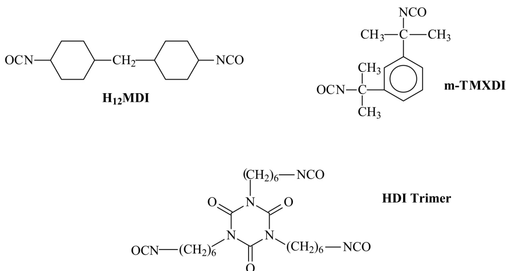
Scheme 1. Common polyisocyanates and their abbreviated names.
