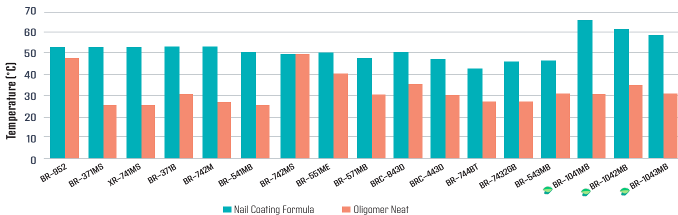
Figure 4. Maximum Temperature Observed During LED Curing
