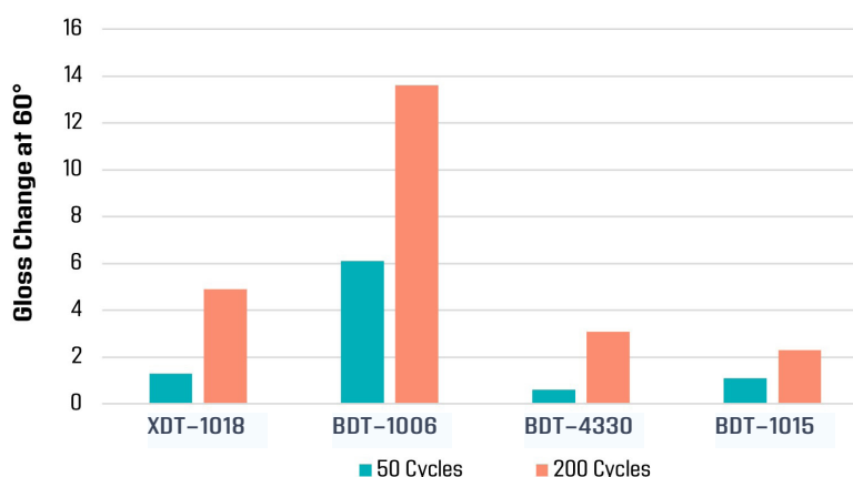
Figure 3. Abrasion Resistance
