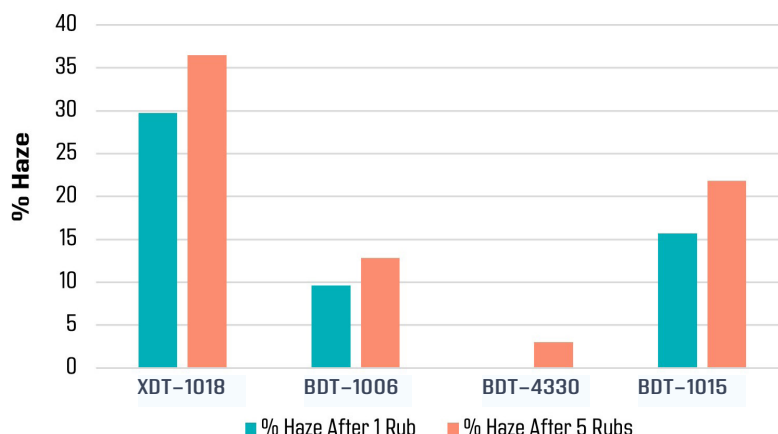
Figure 2. Steel Wool Scratch Resistance
