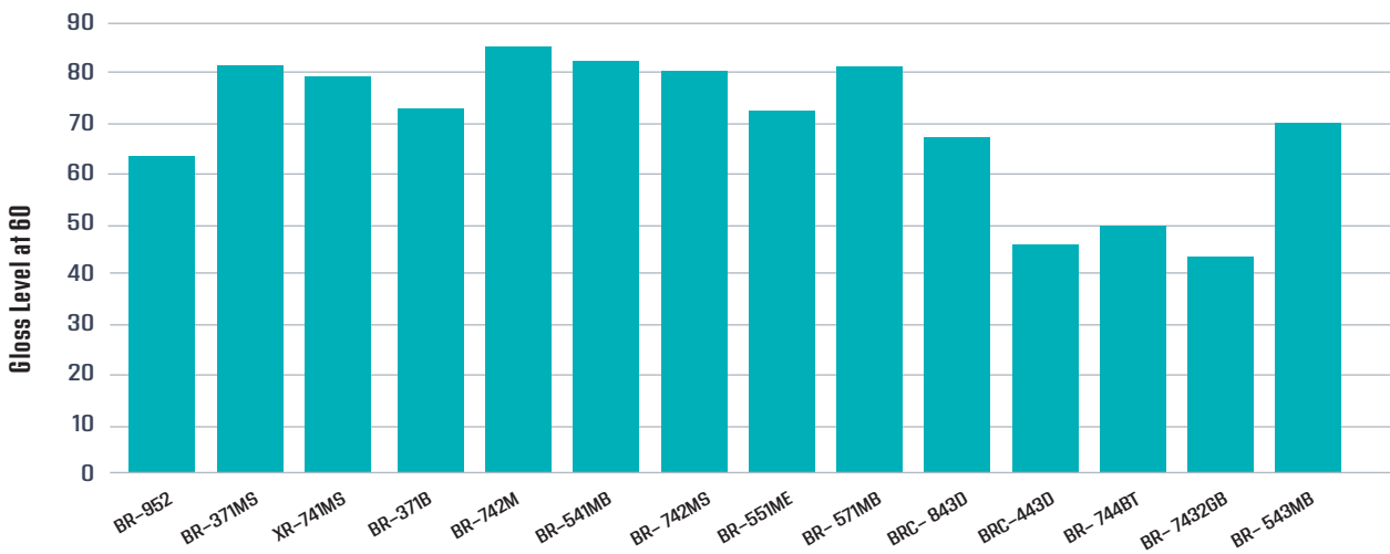
Figure 3. Gloss Coatings after IPA Wipe
