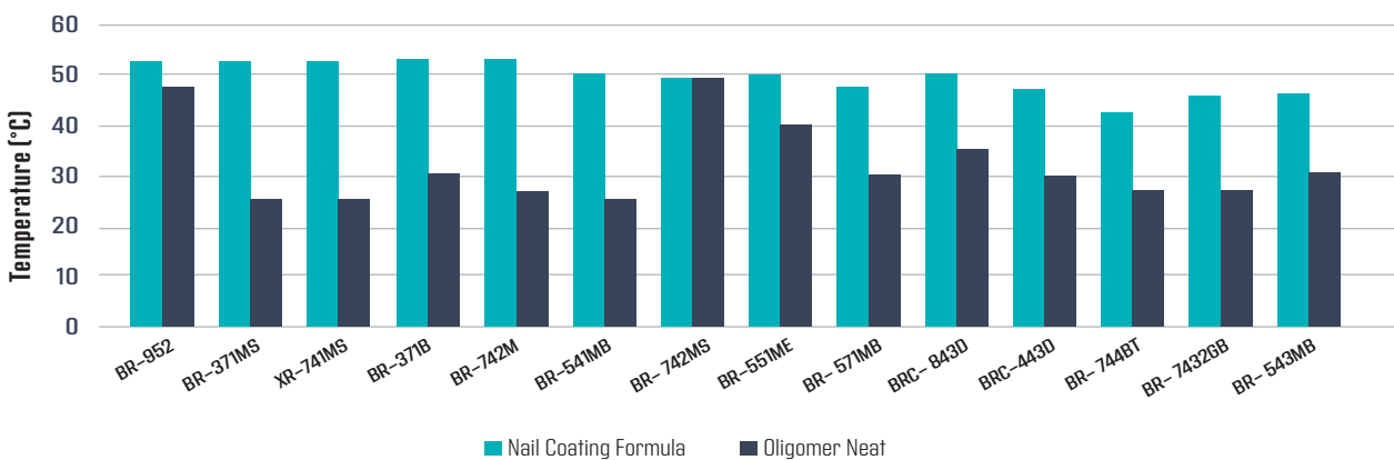
Figure 4. Maximum Temperature Observed During LED Curing
