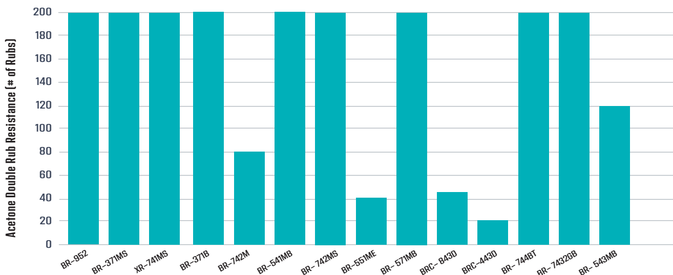
Figure 1. Acetone Double Resistance Provided by the Oligomers
