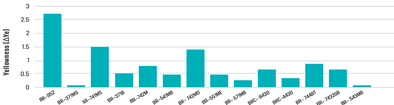
Figure 2. Yellowness Values of the LED-Cured Coatings
