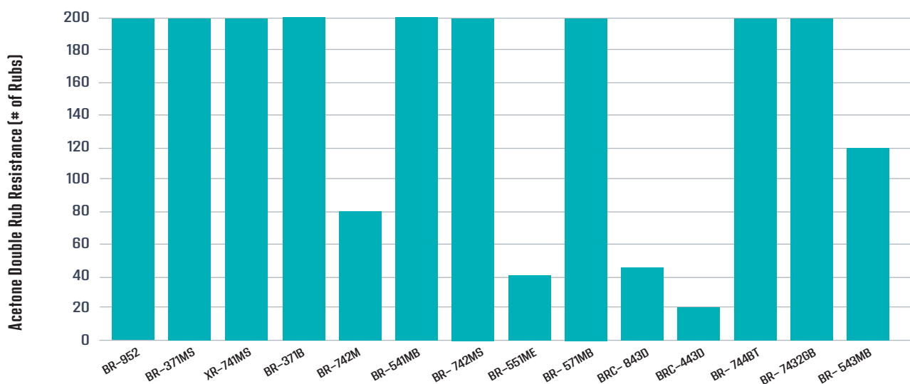
Figure 1. Acetone Double Resistance Provided by the Oligomers
