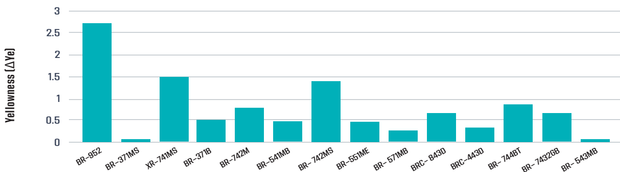
Figure 2. Yellowness Values of the LED-Cured Coatings
